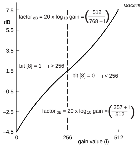
Fig.12 Amplifier curve.
